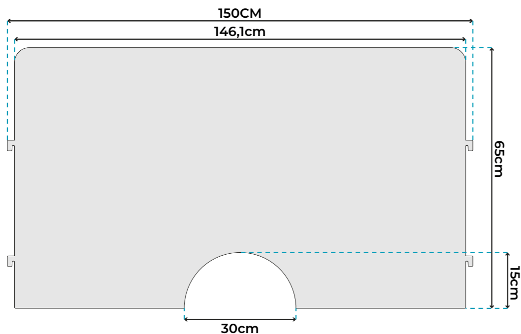
OS-PLEX-150-100-3-O OS-PLEX-150-100-5-O
