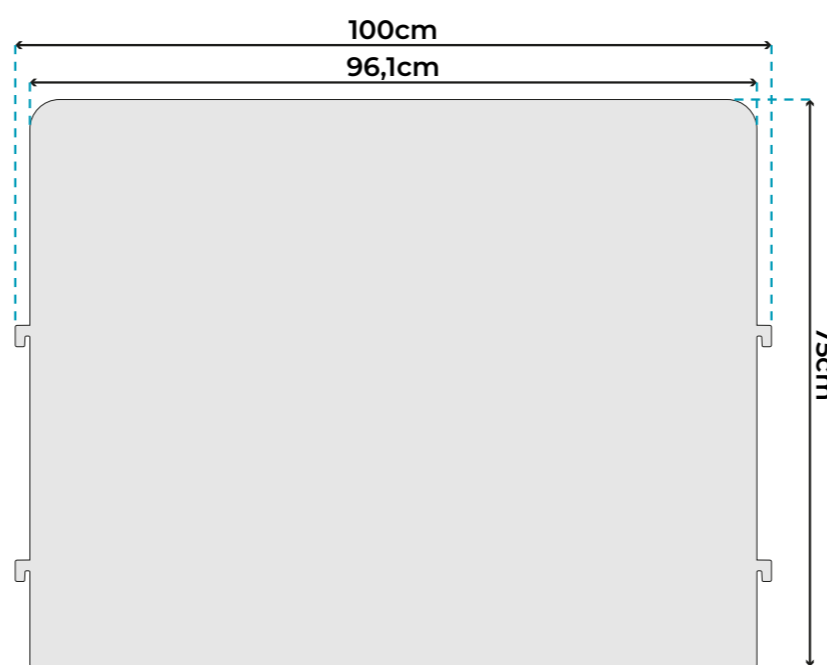
OS-PLEX-100-75-3 OS-PLEX-100-75-5
