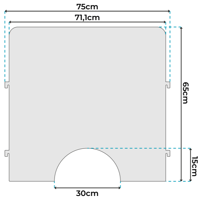
OS-PLEX-75-65-3-O OS-PLEX-75-65-5-O
