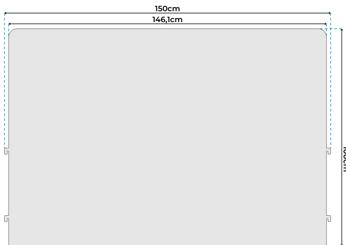
OS-PLEX-150-100-3 OS-PLEX-150-100-5
