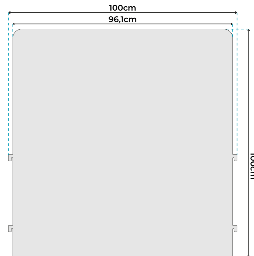
OS-PLEX-100-100-3 OS-PLEX-100-100-5
