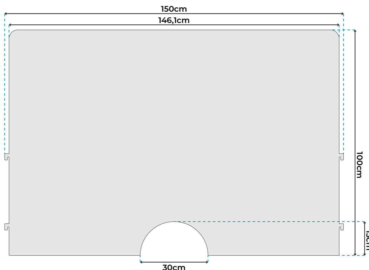
OS-PLEX-150-100-3-O OS-PLEX-150-100-5-O
