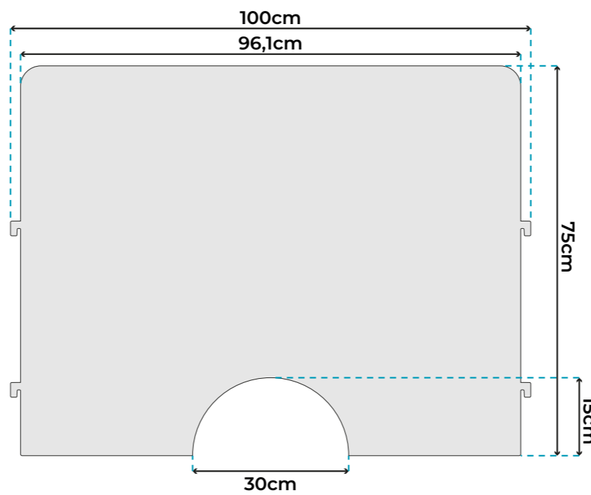
OS-PLEX-100-75-3-O OS-PLEX-100-75-5-O
